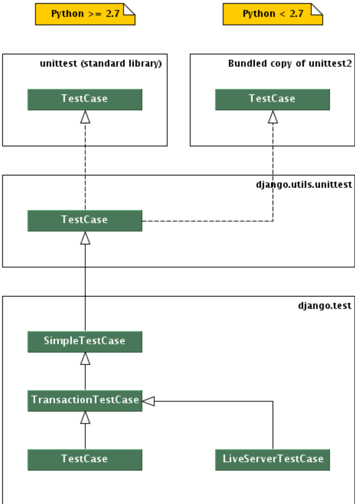
3.9. Testing Django applications Figure 3.1: Hierarchy of Django unit testing classes
